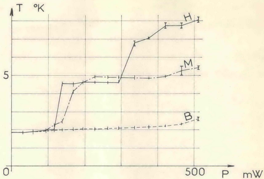
FIG.7 : Superfluid helium T = 1.85 \text{ K} ; p = 2 \text{ atm}
