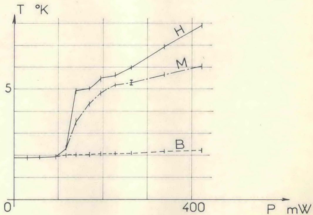
FIG.8 : Superfluid helium T = 1.85 \text{ K} ; p = 3.5 \text{ atm}
